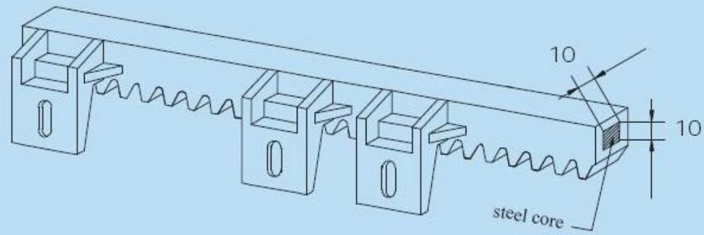
ACRV6 Rack M4 (20x28x1000) with 6 lower overlapped
